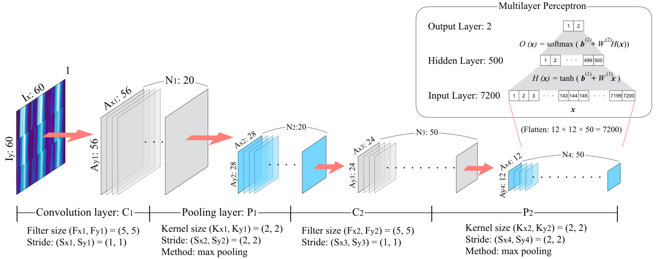
Fig. 2. The overview of the convolutional architecture employed in the fbBCI paradigm. The first convolution layer C_1 generated 20 activation maps (A_{x1}, A_{y1}) = (56, 56) from the input volume matrices (I_x, I_y) = (60, 60) . The consequent pooling layer P_1 conducted a max pooling to the previous activation maps, creating new 20 activation maps (A_{x2}, A_{y2}) = (28, 28) . At the second convolution layer C_2 , 50 activation maps (A_{x3}, A_{y3}) = (24, 24) were created in the same way as the first convolution layer. After that those activation maps were input to the second pooling layer P_2 , generating new 50 activation maps (A_{x4}, A_{y4}) = (12, 12) . Finally, the activation maps generated in the last layer of the convolutional process were flattened into one-dimensional vectors \mathbf{x} ( L = 7200 ) to classify with the one-hidden-layer multilayer perceptron. The flattened vectors \mathbf{x} were conducted two calculations ( H(\mathbf{x}) , O(\mathbf{x}) ) in both input and hidden layers by transforming 7200 units into two units at the output layer.
