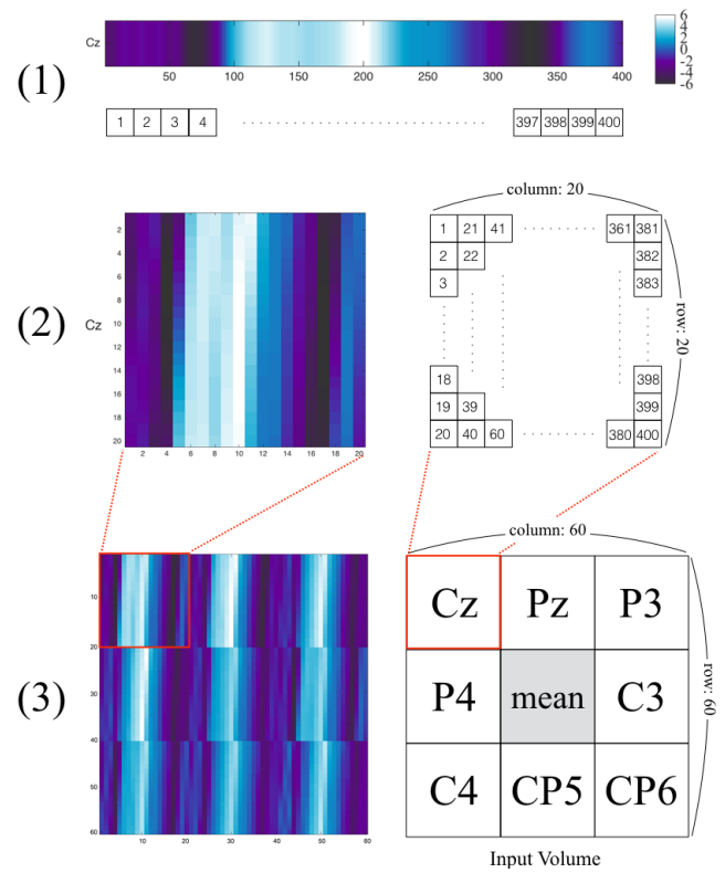
Fig. 1. The generating process of the input volume for the CNN classifier from the signal pre-processed somatosensory ERP intervals in the current study. The each element of the ERP intervals denoted the electrical potential ( \mu V ), the value range of which was shown in the heat map. The sample heat maps in the presented figure signified the mean ERP intervals of target stimulus, so the P300 responses were confirmed around elements number 200 (white colored area), namely around 300 ~ 400 ms ( 200/f_s \approx 0.39 s). The numbers in boxes described in beside of the heat maps were associated with the elements number. (1) Original length of the ERP interval ( ERP_{len} ) was 410, but the first 10 elements were removed to create n \times n squared matrices. (2) The 400 ERP elements were deployed in 20 \times 20. Every 20 elements were placed in vertical direction from top left as shown in the boxes. (3) The 20 \times 20 matrices generated in eight electrode channel and mean of all the electrodes were concatenated in a 3 \times 3 grid pattern for creating 60 \times 60 input volume.
