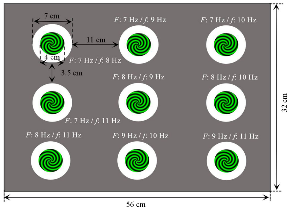
Fig. 1 The layout position of the hybrid paradigm and its corresponding motion frequency and light-flashing frequency
